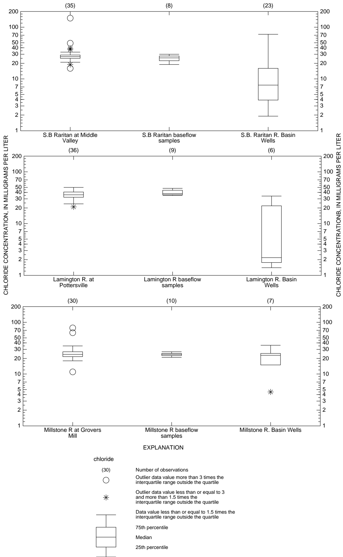
Figure 5. Distribution of chloride concentrations at three stream sites in all samples and in baseflow samples from 1991-97 and at shallow wells located in the drainage basin upstream from the sites from 1985-94
