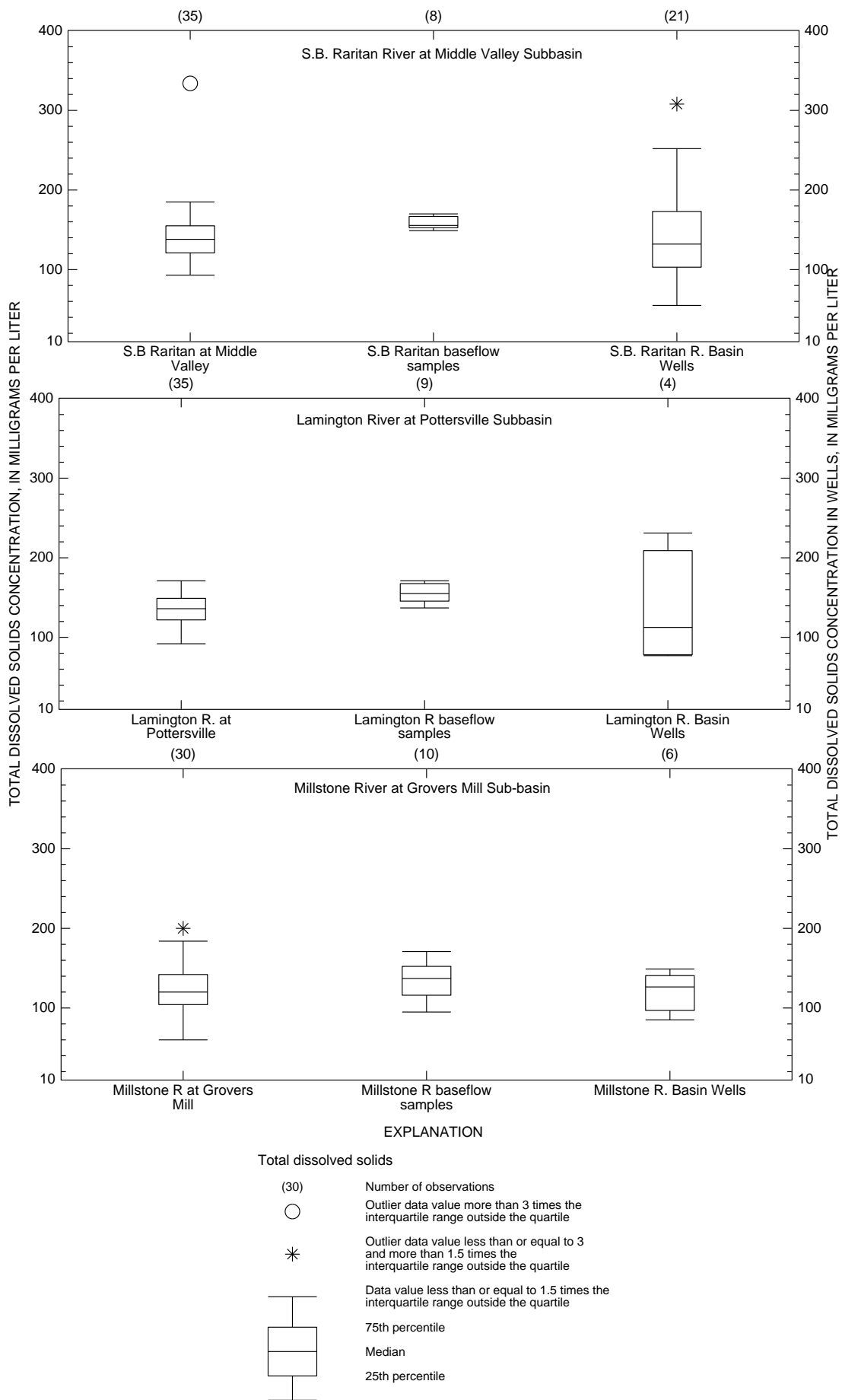
Figure 6. Distribution of total dissolved solids concentrations at three stream sites from all samples and from baseflow samples from 1991-97 and at shallow wells located in the drainage basin upstream from the sites from 1985-94
