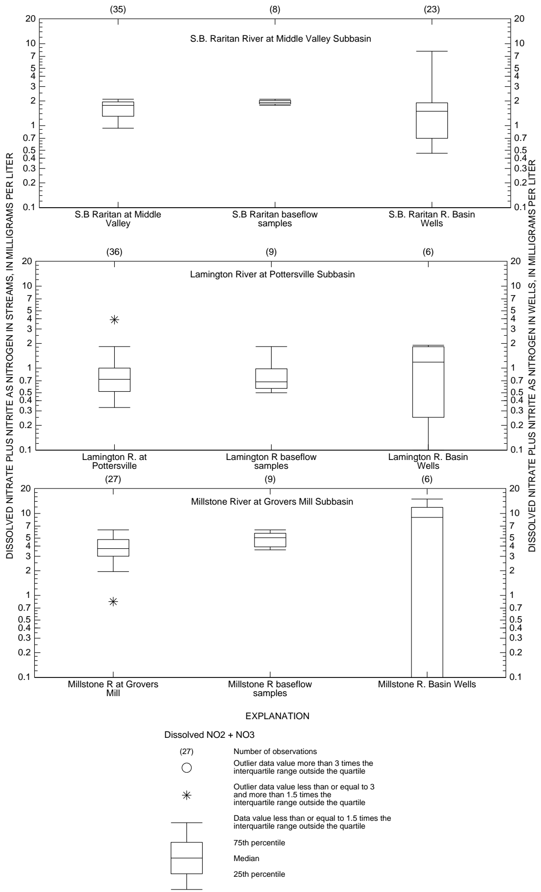
Figure 7. Distribution of dissolved nitrate plus nitrite concentrations at three stream sites from all samples and from baseflow samples from 1991-97 and at shallow wells located in the drainage basin upstream from the sites from 1985-94
