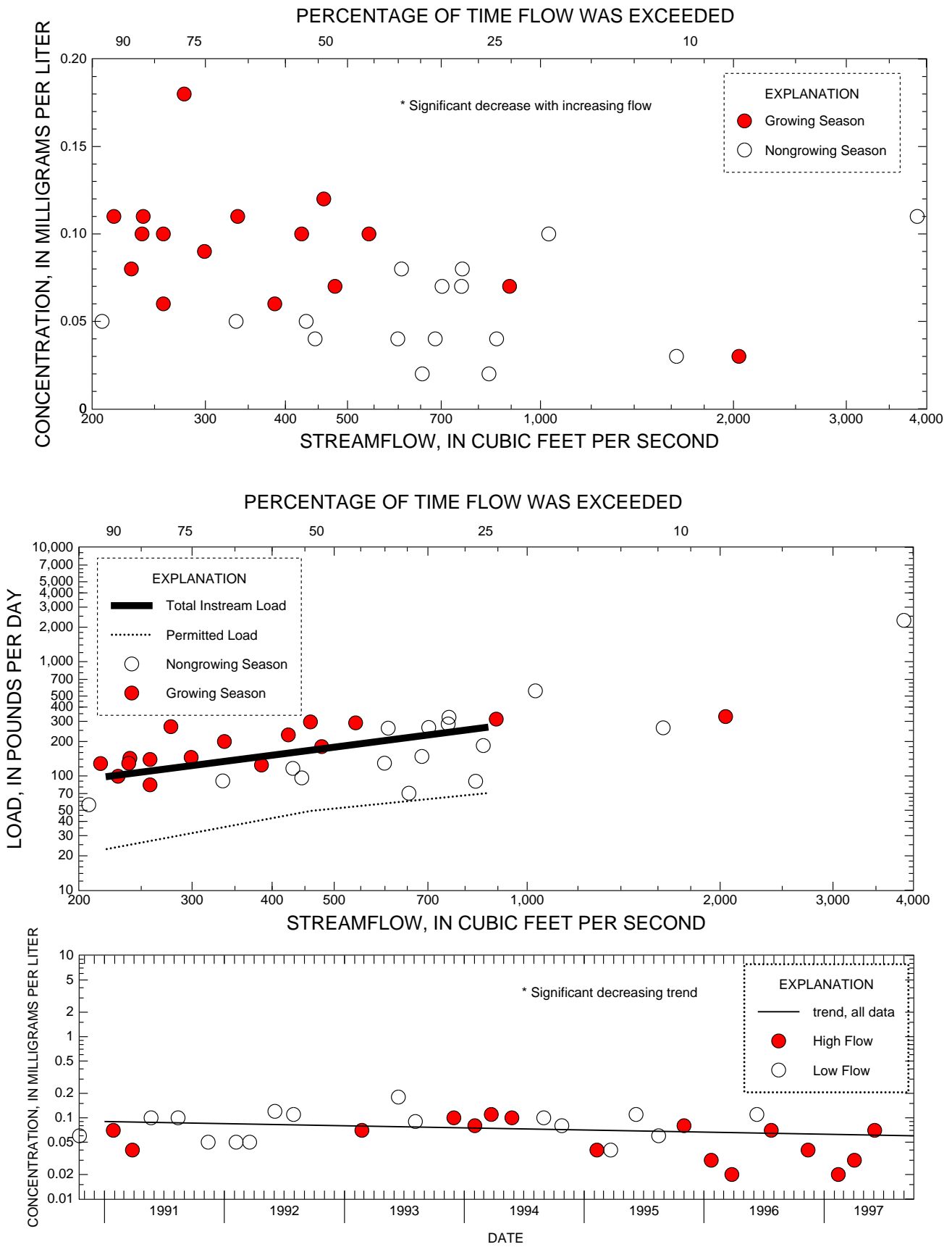
Figure 11. Relation of total phosphorus concentrations and load to streamflow and trends in low and high-flow concentrations at 01400500 Raritan River at Manville, NJ
