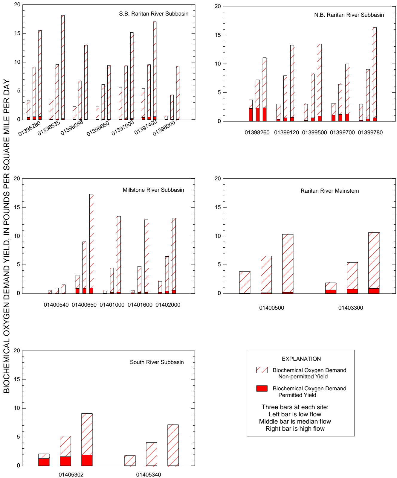
Figure 16. Stacked bar charts showing the permitted and nonpermitted component of total biochemical oxygen demand yield at low, median and high flow conditions
