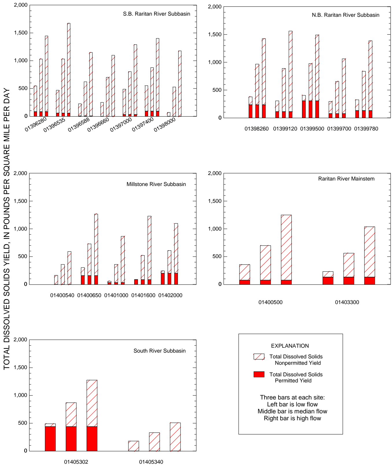
Figure 17. Stacked bar charts showing permitted and nonpermitted components of total dissolved solids yield at low, median, and high flow conditions
