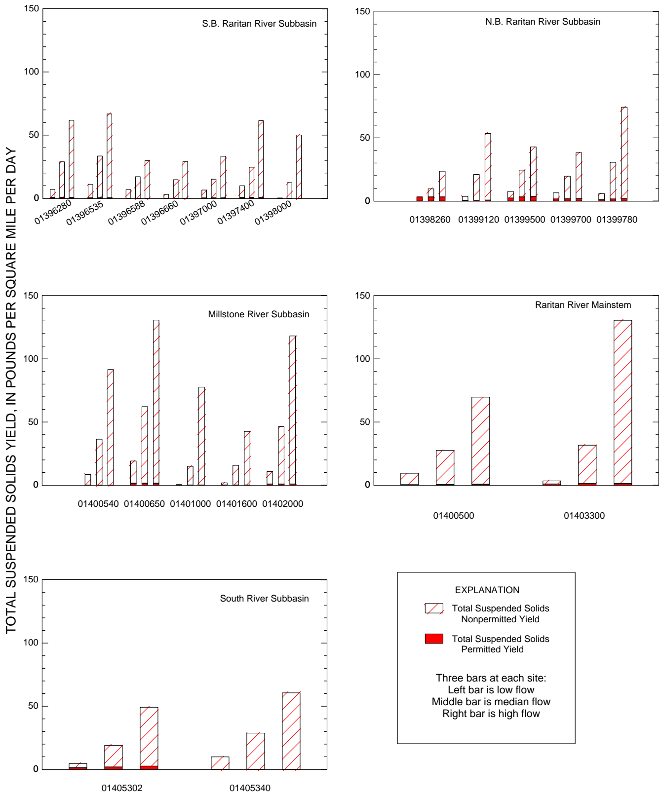
Figure 21. Stacked bar charts showing permitted and nonpermitted components of total suspended solids yield at low, median, and high flow conditions
