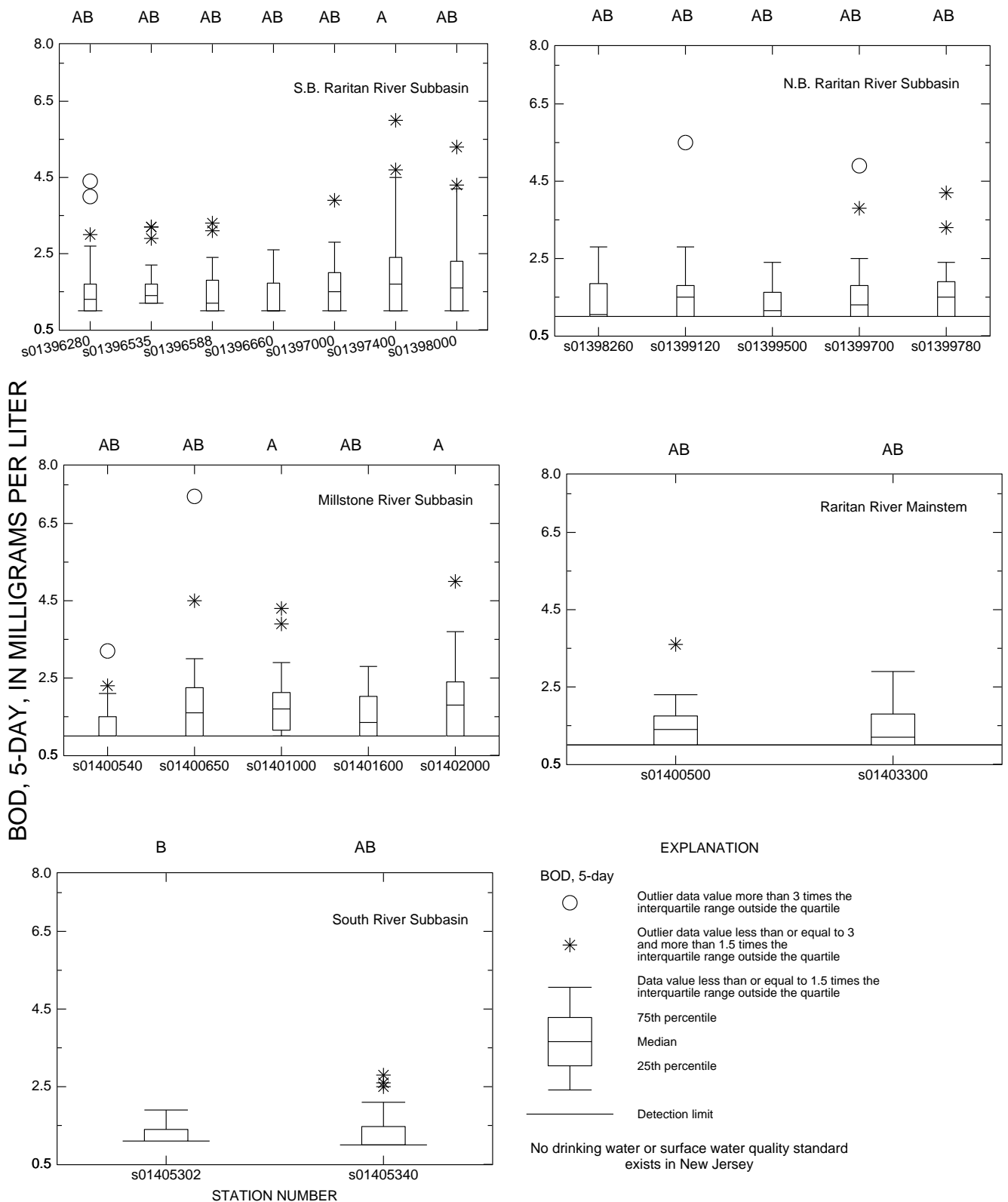
Figure 21. Distribution of biochemical oxygen demand concentrations from samples collected at 21 sites in the Raritan River Basin, 1991-97. [Significant differences in mean rank concentrations between sites from Tukey's test: from A the highest to B the lowest]
