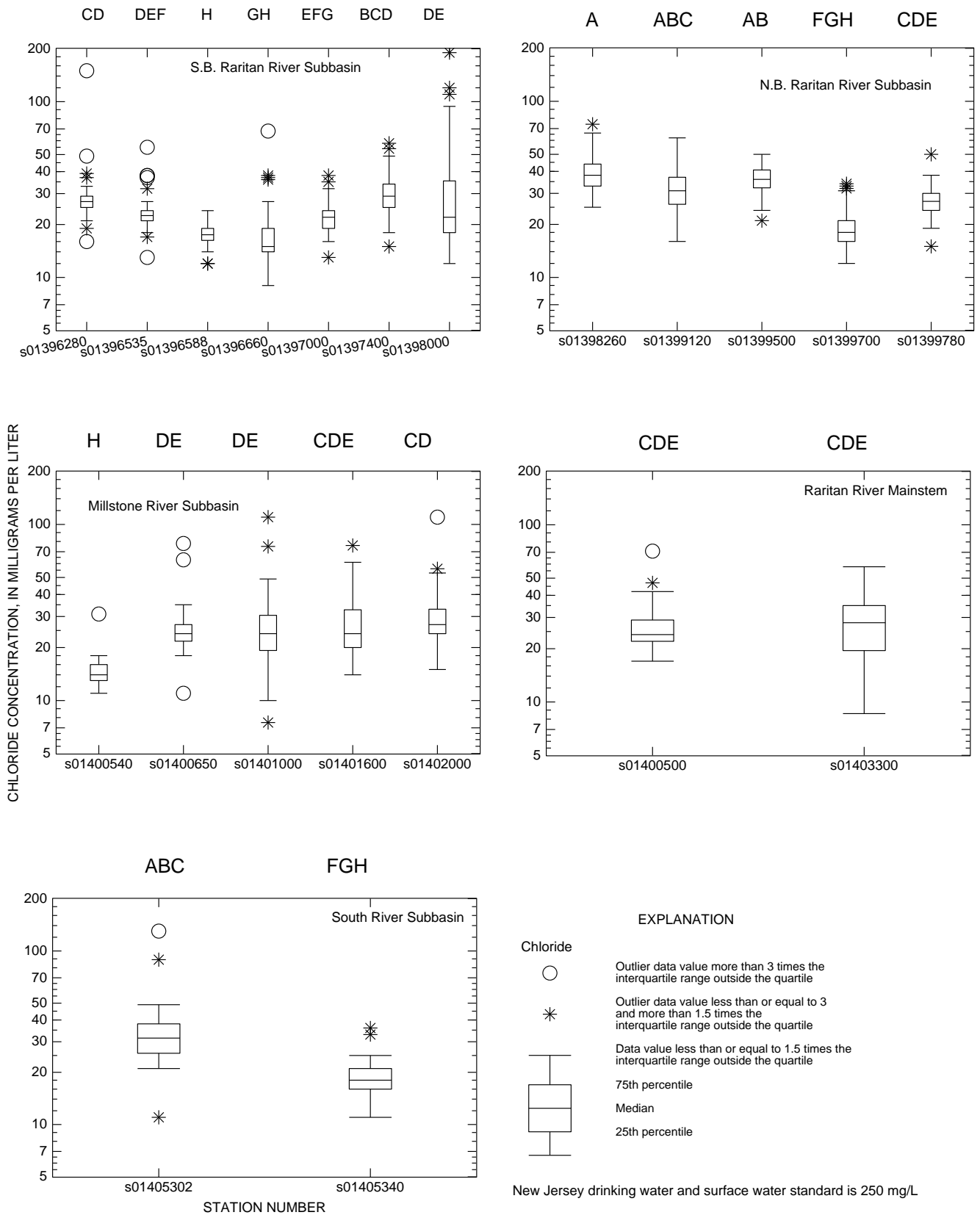
Figure 22 . Distribution of chloride concentrations from samples collected at 21 sites in the Raritan River Basin, 1991-97. [Significant differences in mean rank concentrations between sites from Tukey's test: from A the highest to H the lowest]
