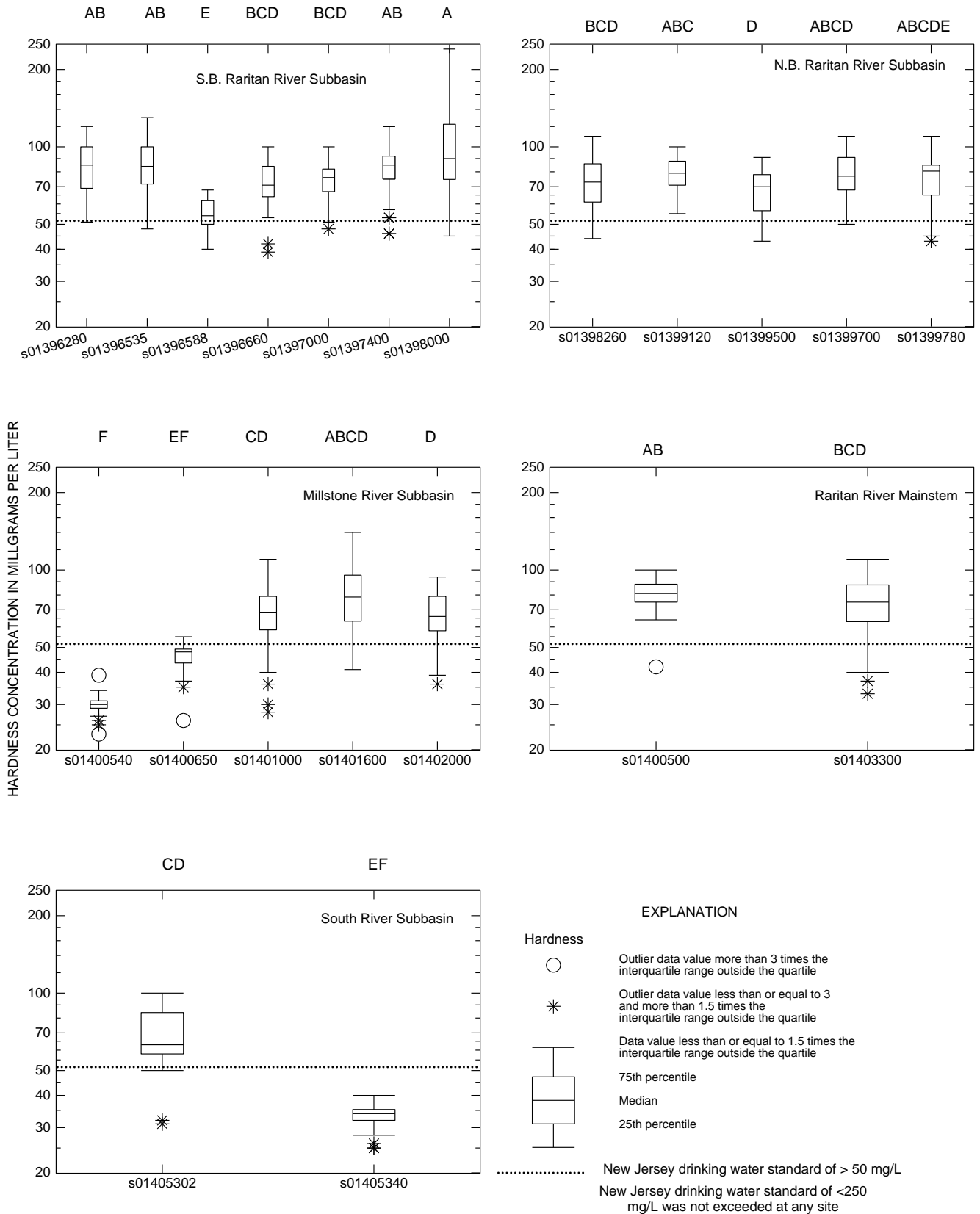
Figure 26. Distribution of hardness concentrations from samples collected at 21 sites in the Raritan River Basin, 1991-97. [Significant differences in mean rank concentrations between sites from Tukey's test: from A the highest to F the lowest]
