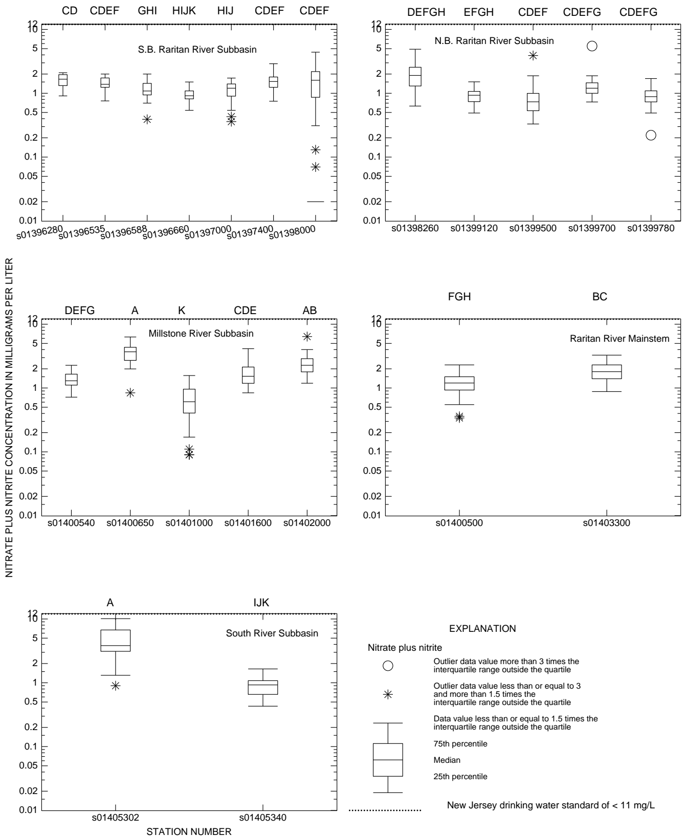
Figure 27. Distribution of nitrate plus nitrite concentrations from samples collected at 21 sites in the Raritan River Basin, 1991-97. [Significant differences in mean rank concentrations between sites from Tukey's test: from A the highest to K the lowest]
