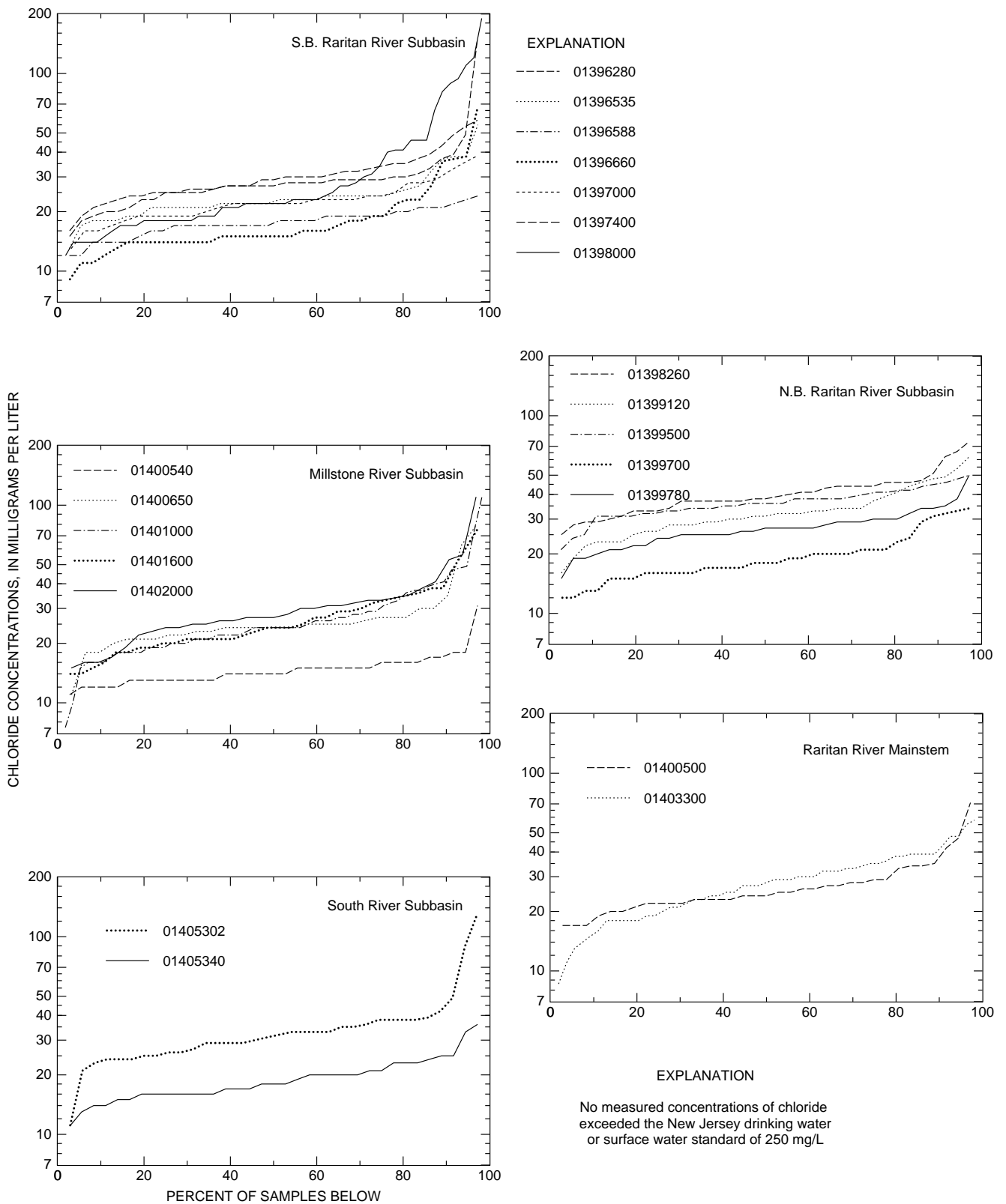
Figure 39 Cumulative probability curve for chloride concentrations from samples collected at 21 sites in the Raritan River Basin, 1991-97
