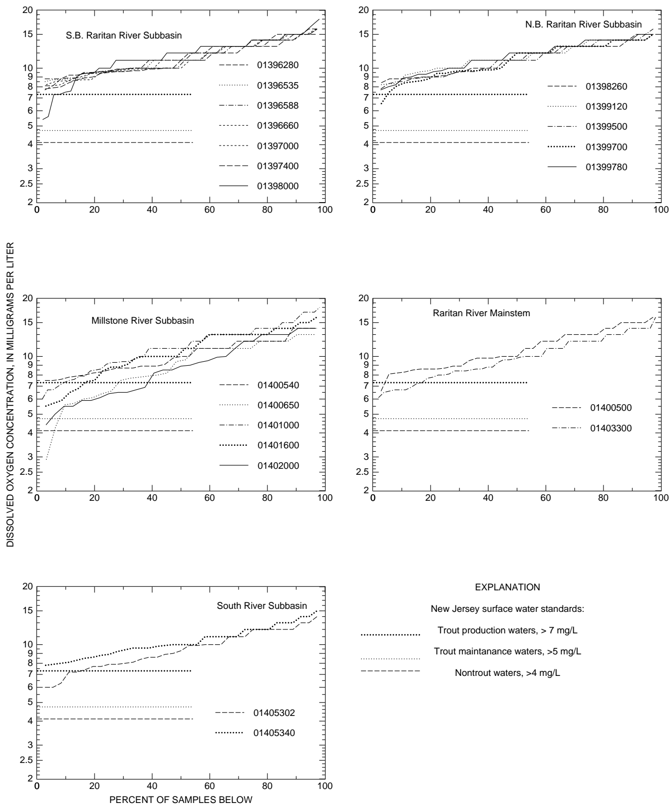
Figure 40. Cumulative probability curve for dissolved oxygen concentrations from samples collected at 21 sites in the Raritan River Basin, 1991-97
