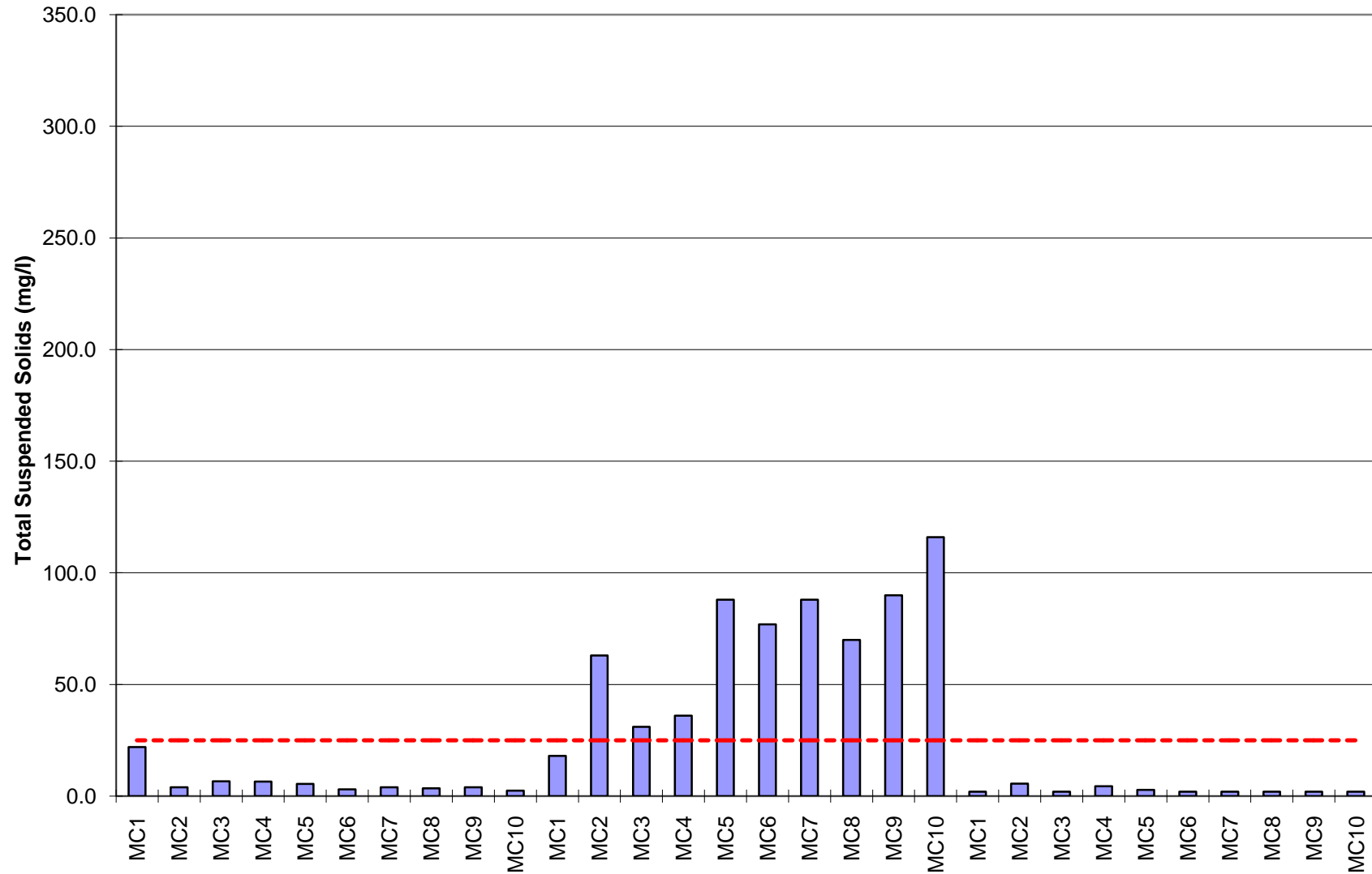
Figure 12. TSS for Storm Event 2: October 16-18, 2006
