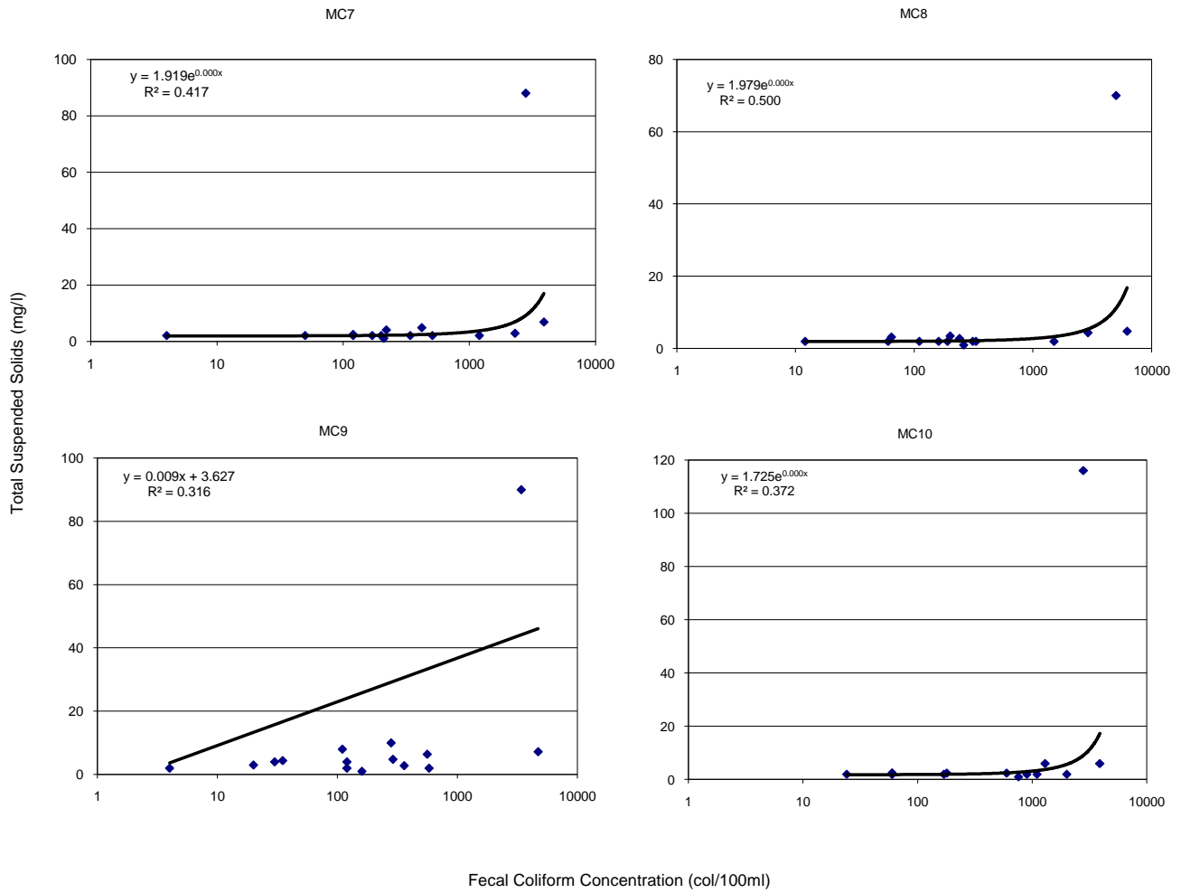
Figure 14. Comparison of Fecal Coliform Concentrations and Total Suspended Solids MC7-MC10
