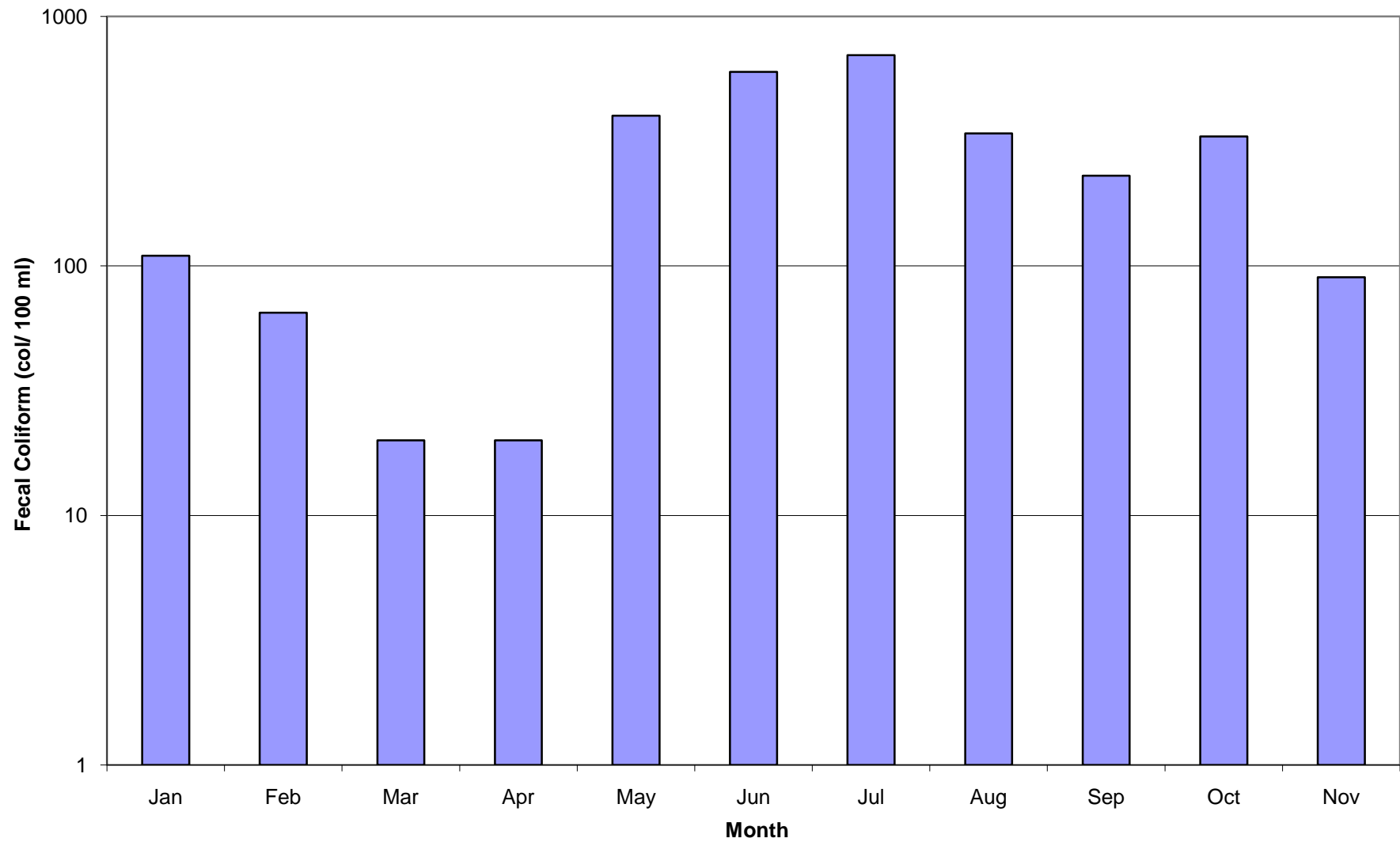
Figure 3. Monthly Median Fecal Coliform Concentrations
