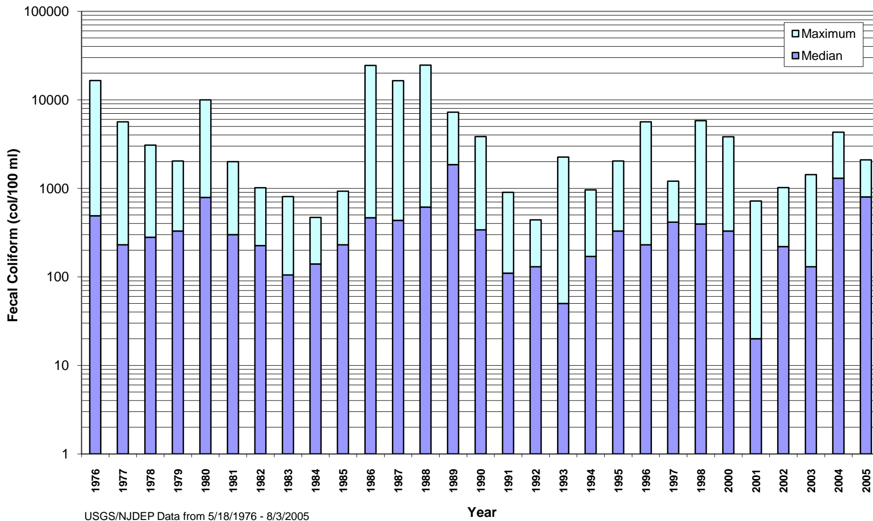
Figure 4. Median and Maximum Annual Fecal Coliform Concentrations at USGS Gauge 01396660 Mulhockaway at Van Syckel
