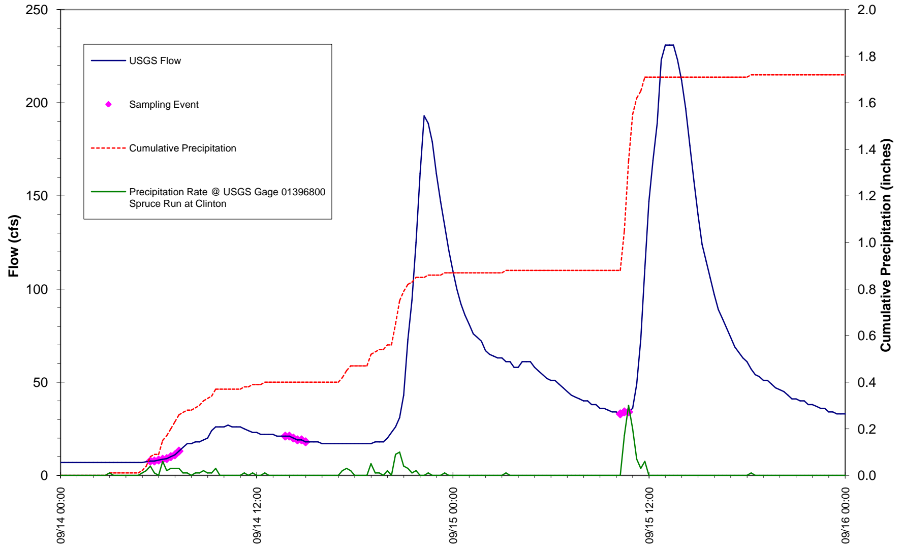
Figure 6. Hydrograph, Precipitation and Sample Times for Storm Event #1
