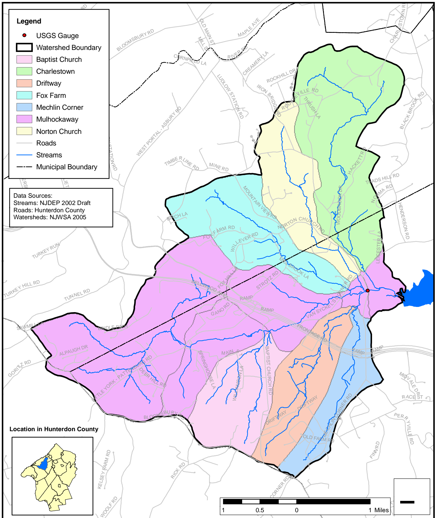
Figure 2. Watershed Hydrography
