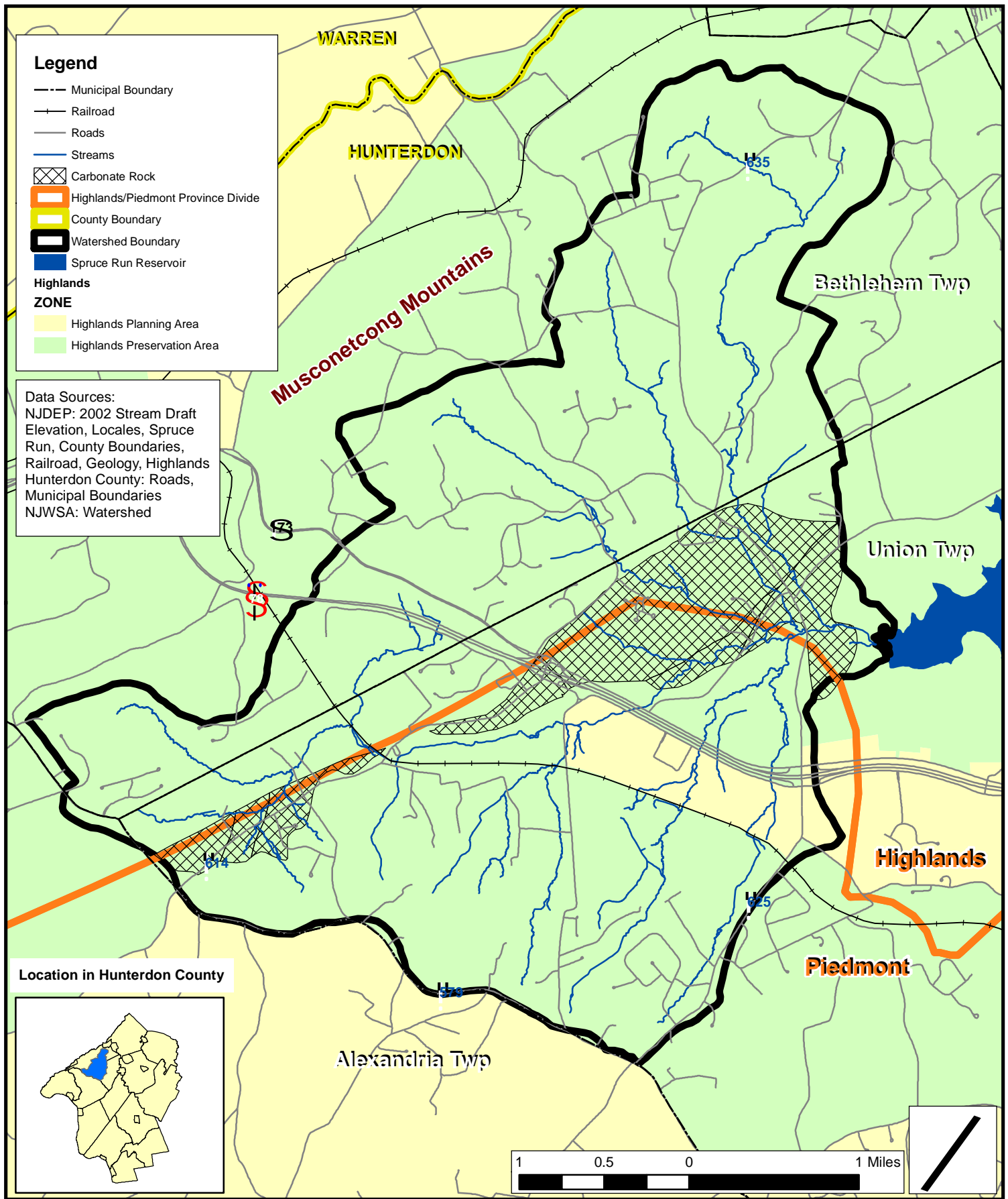
Figure 3. Geology and Highlands Zones
